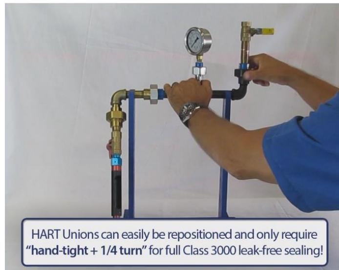
HART Flat-Faced O-Ring design makes pipe alignment easy since it is unnecessary to spring the line during make-up or disassembly!
