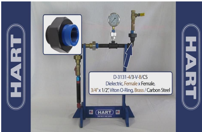
Import-Style Ball/Cone Union
